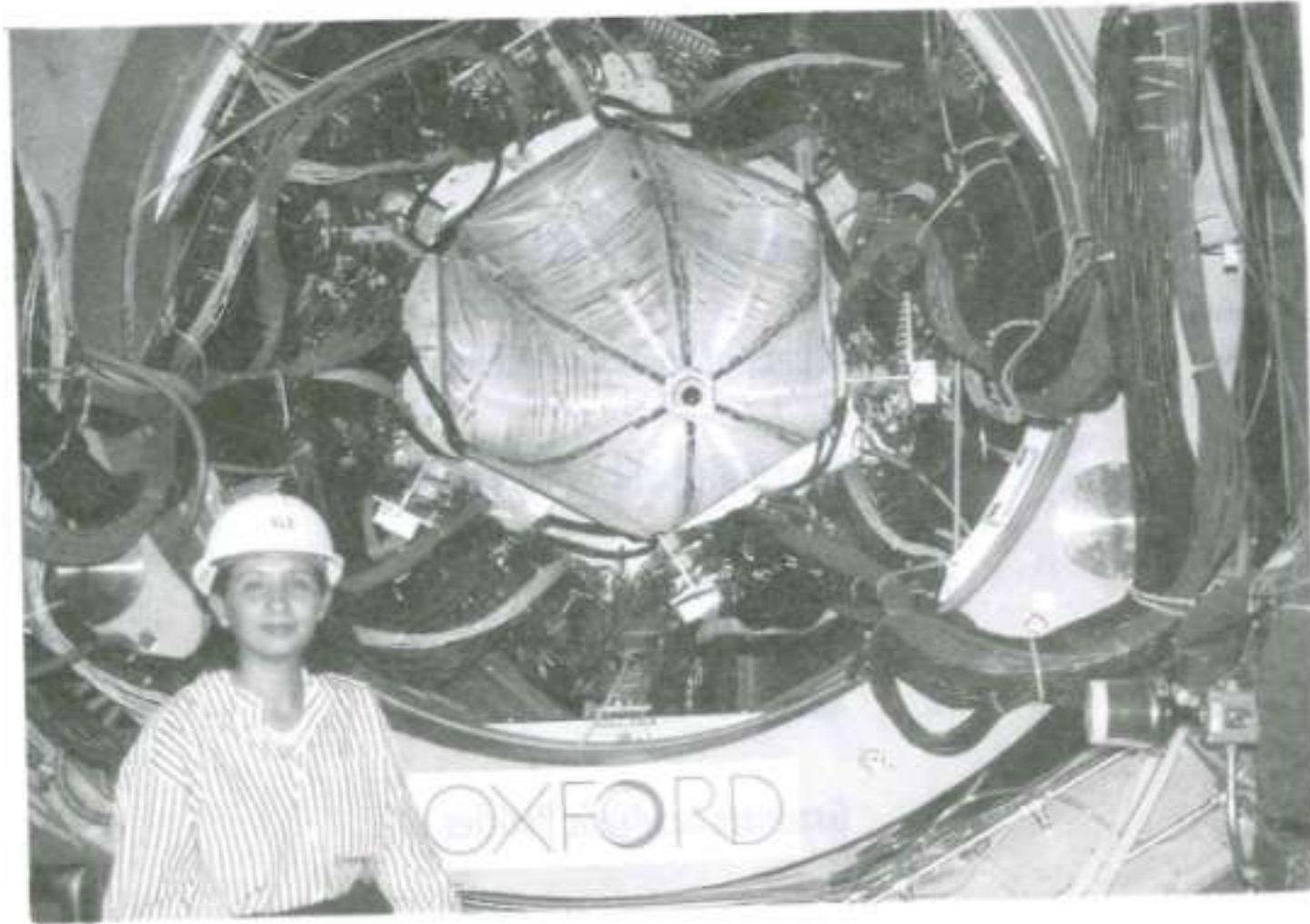
CNU's graduate faculty member Dr. Latifa Elouadrhiri is also a researcher at the Thomas Jefferson National Accelerator Facility. This is a photograph of Dr. Elouadrhiri next to the CLAS detector. The drift chambers are visible at the center of the opening.
